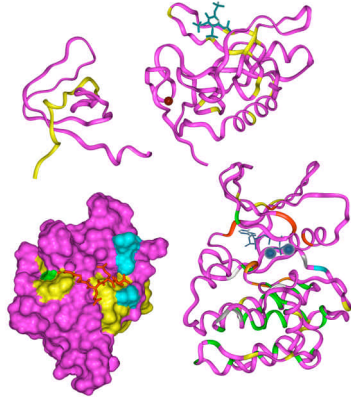
Figure 2. Three-dimensional structures of Btk domains. Top left, Btk SH3 domain. The inframe deletion of the C-terminus of the domain is shown in yellow. Top right, Btk PH domain. The locations of the XLA-causing missense mutations (yellow) are concentrated mainly on the phosphatidylinositol (green) binding site region. Zn^{2+} is in cyan. Bottom left, Btk SH2 domain model. The disease-causing mutations are in yellow. Ligand peptide is in blue. Bottom right, Btk kinase domain model with color coded consequences of missense mutations. The putative structural alterations are in green, ATP binding site mutations in red, catalytic residues in gold, substrate binding site mutations in white, the phosphotyrosine binding site in cyan, and domain-domain or protein-protein interaction sites in yellow. ATP and Mg^{2+} ions are in cyan.
