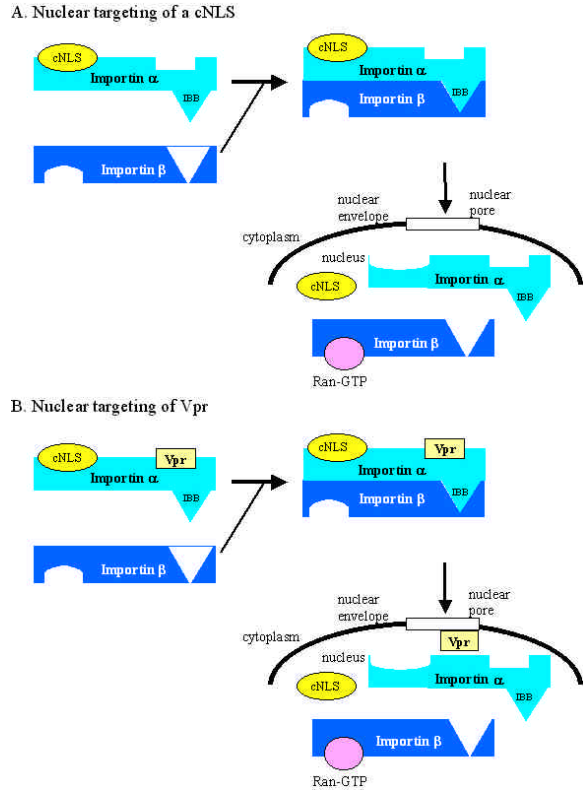
Figure 2. Nuclear localization. (A) Nuclear targeting of a cNLS. (B) Nuclear targeting of Vpr.
