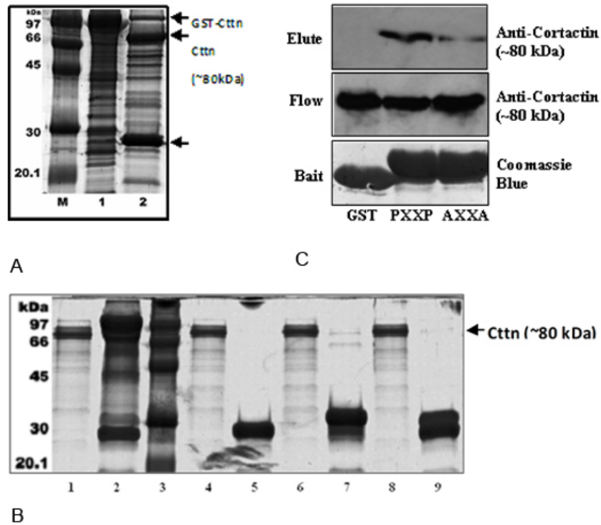
Figure 3. Immunoprecipitation of full-cortactin by HBx. (A) Cortactin was cloned as a GST-fusion protein in pGEX-5X-1 (GST-Ctnn) and properly expressed (lane 1) GST moiety was removed (lane 2) to obtain purified cortactin (Ctnn) (B) GST and GST-Ctnn (undigested) were removed by immunoprecipitation, leaving the lysates with cortactin for use in GST pull-down analysis (lane 1) Lane 2 represents the crude GST-Ctnn extract while Lane 2 signifies the protein rainbow marker RPN756 (GE Healthcare) GST (negative control), GST-PXXP and GST-AXXA were first immunoprecipitated. HBx PXXP region binds cortactin (Lane 7) but not GST-AXXA (Lane 9) No binding was observed with GST alone (Lane 5) Lanes 4, 6 and 8 represents the equal loading of Ctnn for interaction purposes. (C) GST pull-down system (GST, GST-PXXP and GST-AXXA as bait) for endogenous cortactin using lysates of HepG2 cells were performed. Endogenous cortactin was detected by anti-cortactin antibody.
